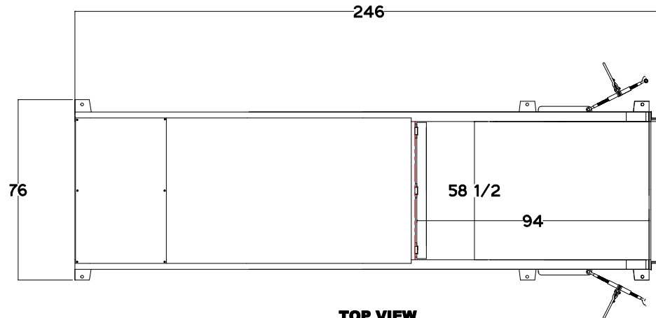
TOP VIEW
