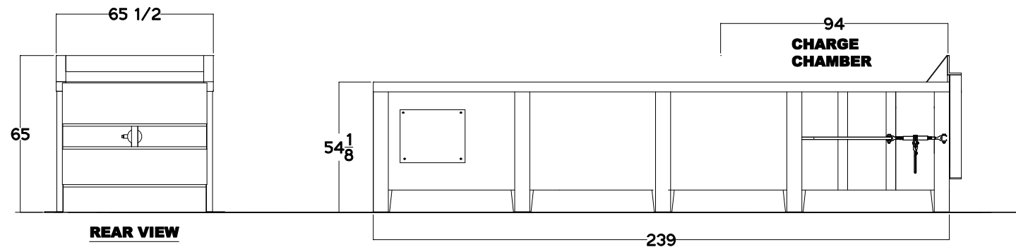
SIDE VIEW
